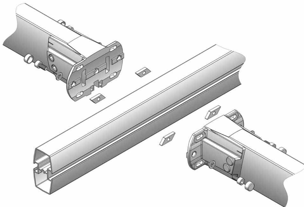
GUIDE PROFILE WITH DOUBLE SPACE FOR ADJUSTMENTS PROFIL DE GUIDAGE RÉGLETTE DOUBLE
