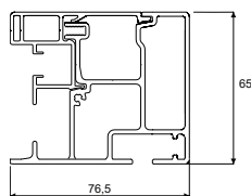
Guide rail
