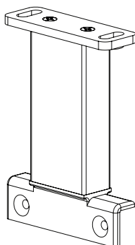
Support foot 2
