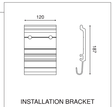
Detail D
